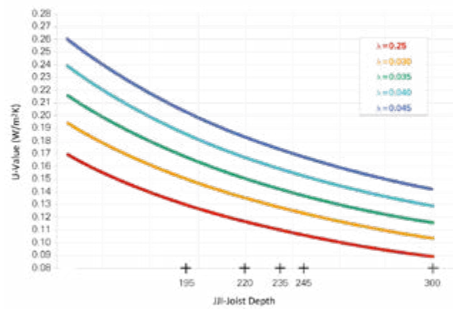
Indicative U-Values for typical JJI-Joist Stud External Wall
